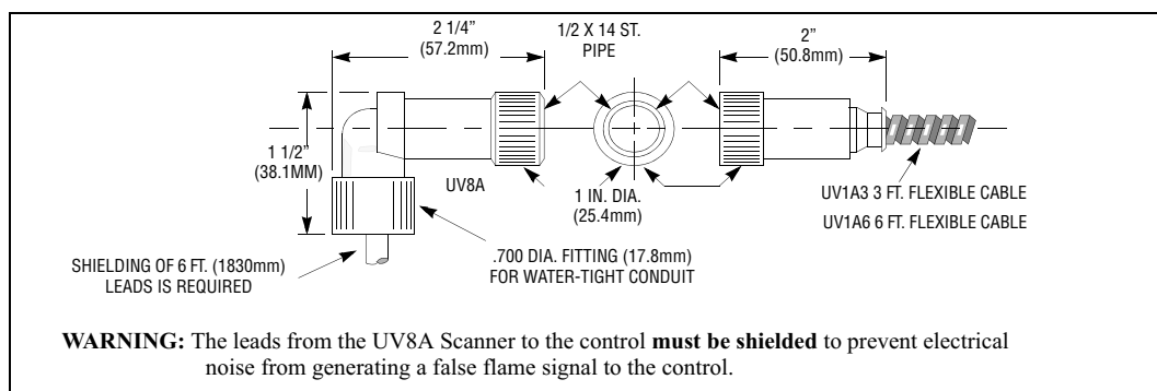
FIGURE 17. UV8A Scanner
