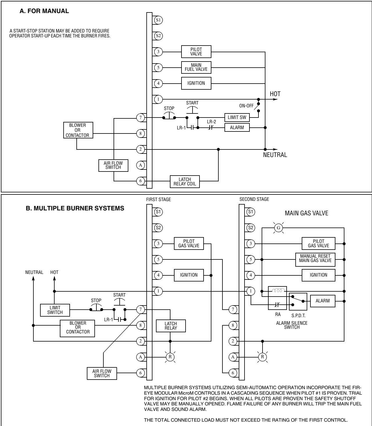
FIGURE 13. ALTERNATE WIRING ARRANGEMENT FOR MEP CONTROLS
