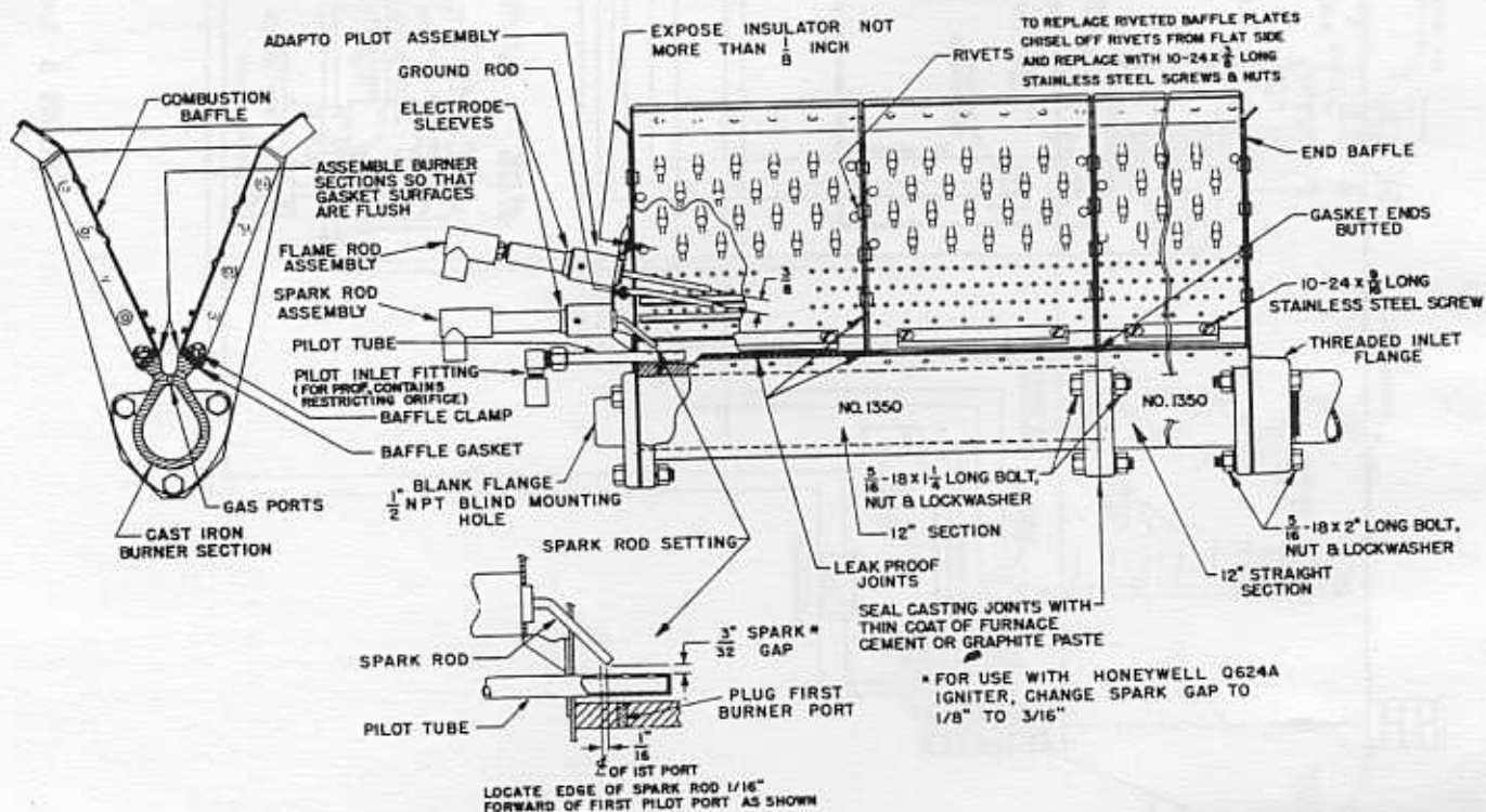
FIGURE 7 BURNER ASSEMBLY
