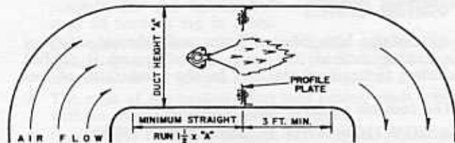
FIGURE 4 ELBOW DUCTS LIMITS
