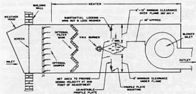
FIGURE 2 INSTALLATION IN HEATER
