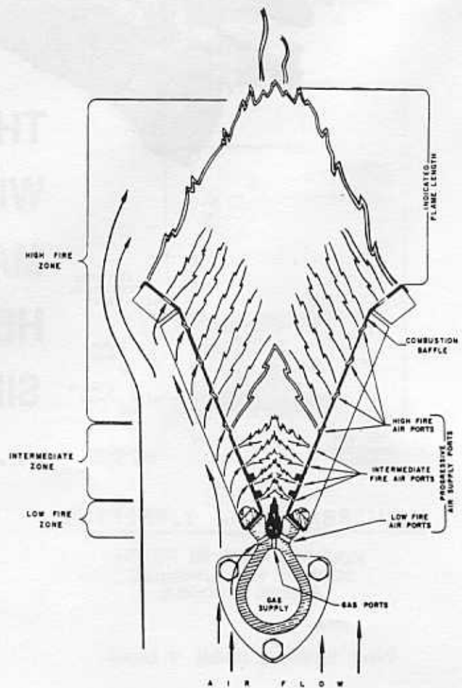
FIGURE 1 COMBUSTION PATTERN
