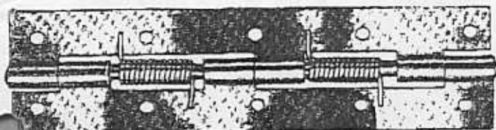
H2013-.060 x 1-1/2" x 5-3/8" x .156 .140 dia. holes on 1-3/16 centers
