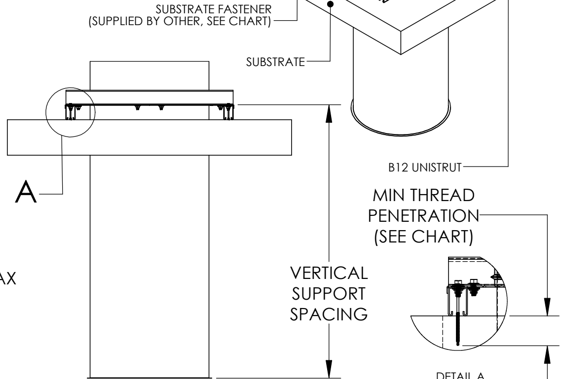
DETAIL A SCALE 1 : 8
