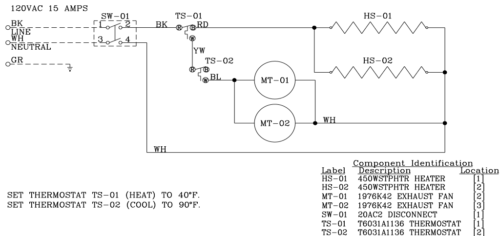
Typical Wiring Schematic for the Climate Controlled Utility Cabinet
